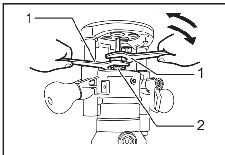
▶ 1. Wrench 2. Collet chuck
